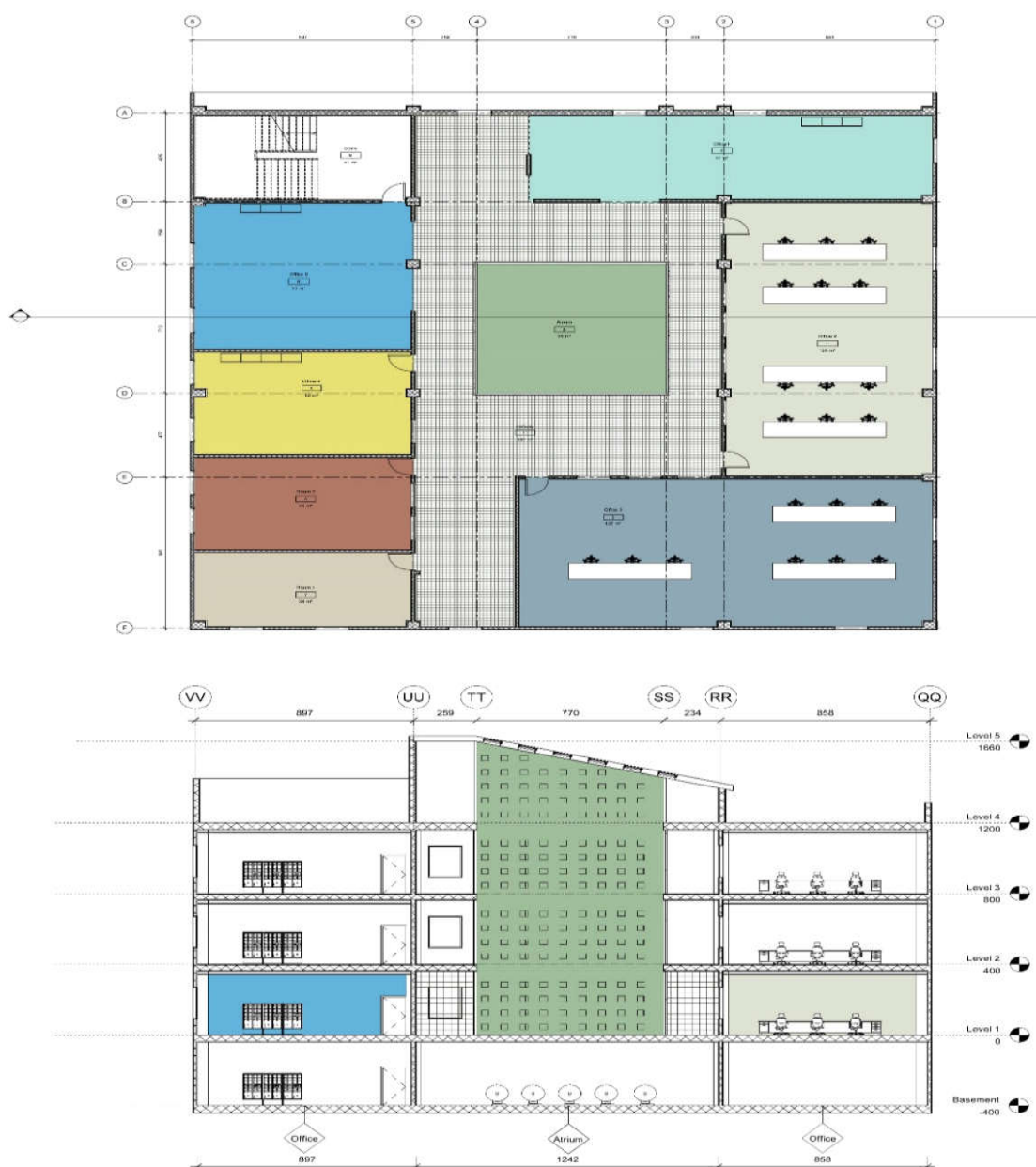
Fig. 1: Floor plan (above) and cross section (below) of the atrium
